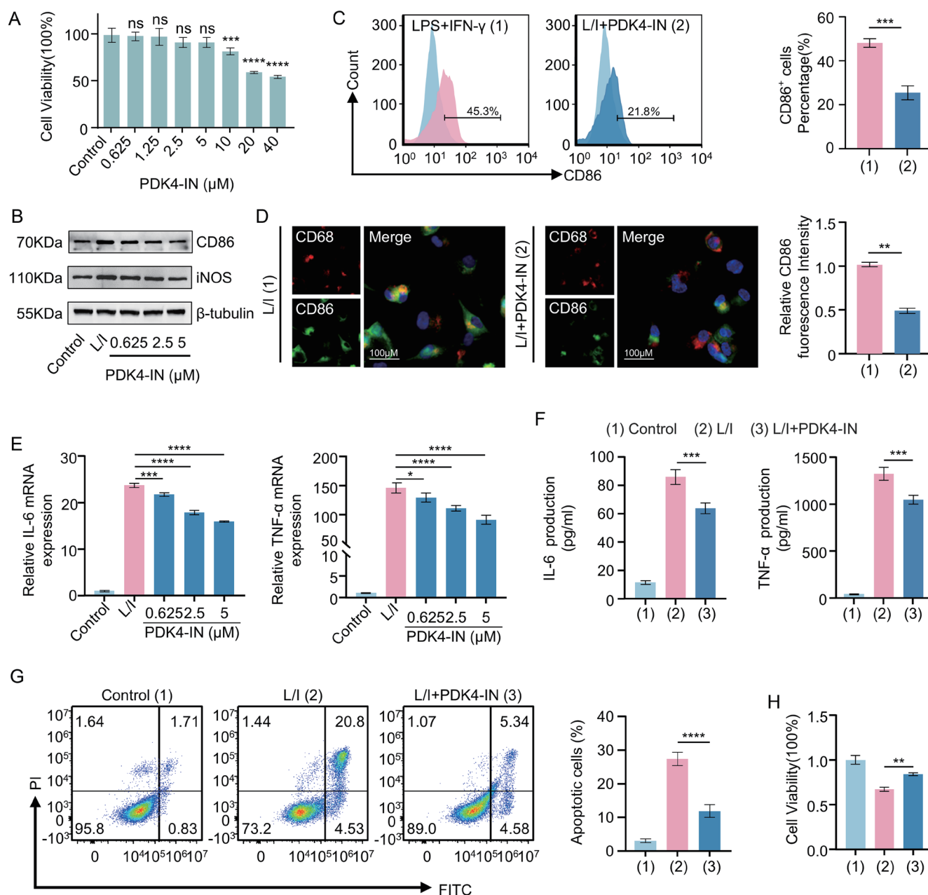
Fig. 5. Effects of PDK4 inhibition on M1 polarization in THP-1 macrophages and hepatocyte injury. (A) Cell viability of THP-1 macrophages treated with increasing concentrations of PDK4-IN (0–40 \mu M) for 24 h was assessed by CCK-8 assay. (B) Protein levels of the M1 markers CD86 and iNOS were analyzed by Western blot. (C) The proportion of CD86 + cells was determined by flow cytometry. (D) CD68 (red) and CD86 (green) expression was visualized by immunofluorescence staining; nuclei were counterstained with DAPI (blue); scale bar = 100 \mu m. Quantification of fluorescence intensity is shown on the right. (E) mRNA expression of IL-6 and TNF- \alpha was measured by RT-qPCR. (F) Secreted levels of IL-6 and TNF- \alpha in the supernatant were quantified by ELISA. (G) Flow cytometric analysis of apoptosis in LO2 cells cultured with conditioned media derived from macrophages. (H) CCK-8 assay of viability in LO2 cells cultured with conditioned media derived from macrophages. Data are presented as mean \pm SD (n = 3). Statistical significance was determined by unpaired two-tailed Student's t-test (for comparisons between two groups) or one-way ANOVA (for comparisons among multiple groups). ns, P > 0.05 , * P < 0.05 , ** P < 0.01 , *** P < 0.001 , **** P < 0.0001 . PDK4-IN, pyruvate dehydrogenase kinase 4 inhibitor; CCK-8, Cell Counting Kit-8; CD86, cluster of differentiation 86; iNOS, inducible nitric oxide synthase; IL-6, interleukin-6; TNF- \alpha , tumor necrosis factor- \alpha ; LPS, lipopolysaccharide; IFN- \gamma , interferon- \gamma ; DAPI, 4',6-diamidino-2-phenylindole; ns, not significant.
