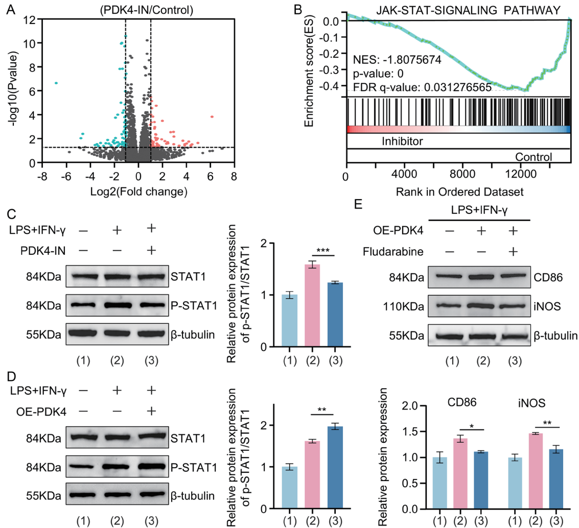
Fig. 6. Effects of PDK4 inhibition or overexpression on STAT1 phosphorylation and M1 polarization in macrophages. (A) Volcano plot showing DEGs in macrophages stimulated with LPS/IFN- \gamma , with or without pretreatment with PDK4-IN. Upregulated genes are shown in red, downregulated genes in cyan. (B) GSEA of transcriptomic data. (C, D) Western blot analysis and quantification of total STAT1 and p-STAT1. Cells were pretreated with either PDK4-IN or PDK4 overexpression vector, followed by LPS/IFN- \gamma stimulation. (E) Western blot analysis and quantification of M1 polarization markers CD86 and iNOS under PDK4 overexpression in the presence or absence of the STAT1 inhibitor fludarabine. Data are presented as mean \pm SD ( n = 3 ). Statistical significance was determined by one-way ANOVA followed by Tukey's post hoc test. * P < 0.05 , ** P < 0.01 , *** P < 0.001 . +, with; -, without; PDK4, pyruvate dehydrogenase kinase 4; STAT1, signal transducer and activator of transcription 1; p-STAT1, phosphorylated STAT1; DEGs, differentially expressed genes; GSEA, gene set enrichment analysis; LPS, lipopolysaccharide; IFN- \gamma , interferon-gamma; CD86, cluster of differentiation 86; iNOS, inducible nitric oxide synthase.
